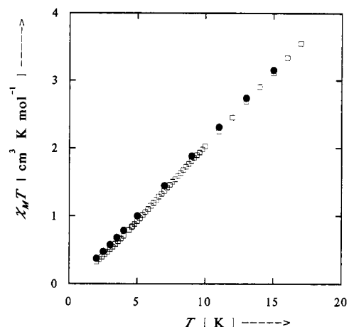
Figure 4. Plot of \chi_M T vs temperature data for a polycrystalline sample of K_4[Mn_{18}O_{16}(O_2CPh)_{22}(phth)_2(H_2O)_4] ( 5 ). Ac magnetic susceptibility data (□) measured in zero dc field with a 1.0 G ac field oscillating at 50 Hz are plotted. The dc data (●) are shown for comparison purposes.
